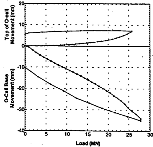
Osterberg Cell Load-Movement Curves
